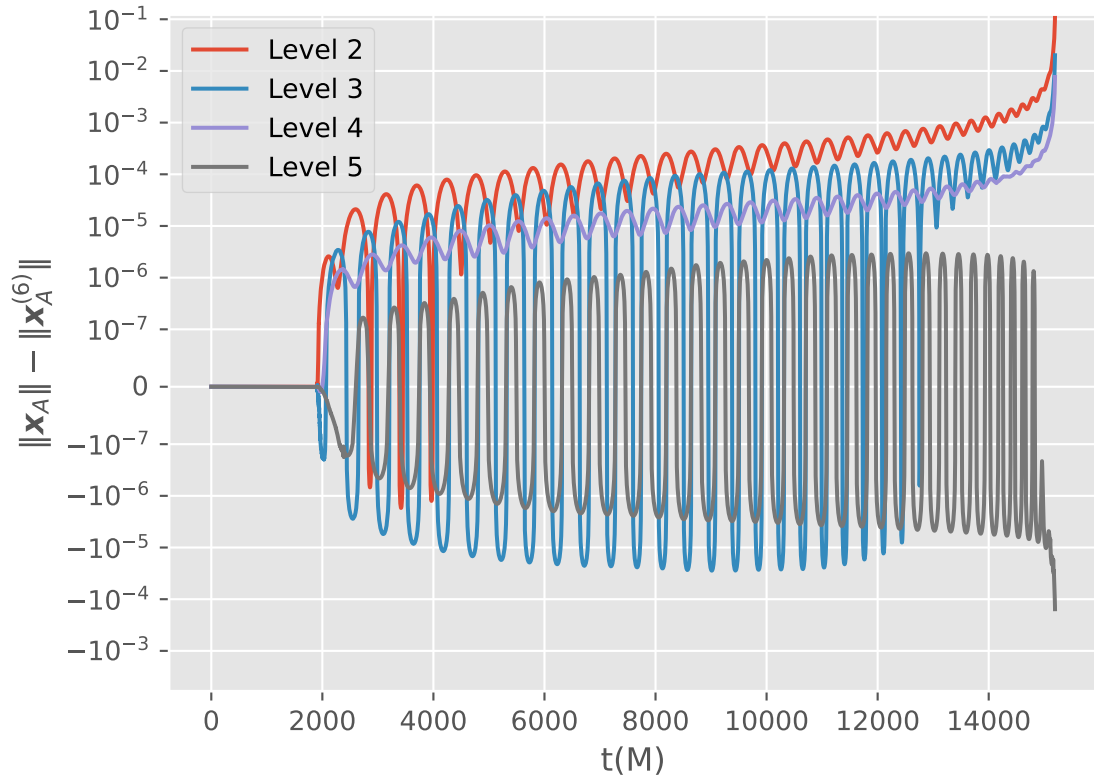
Difference in centers of black hole A for Sim09
