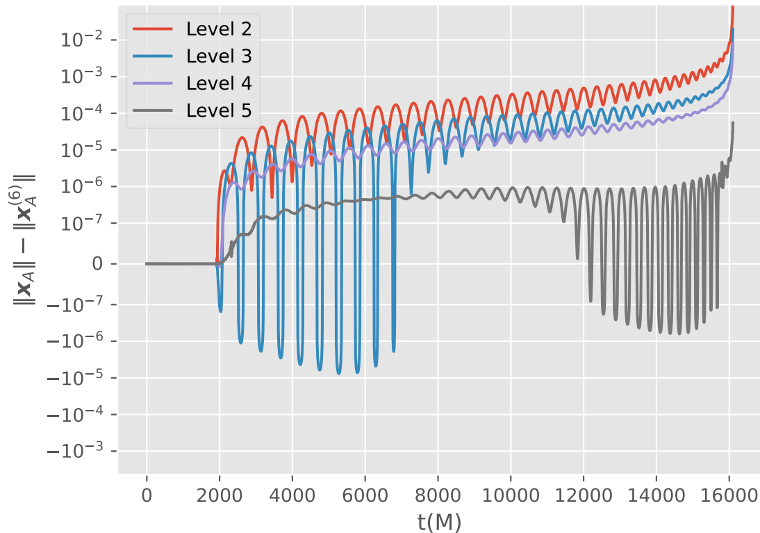
Difference in centers of black hole A for Sim10
