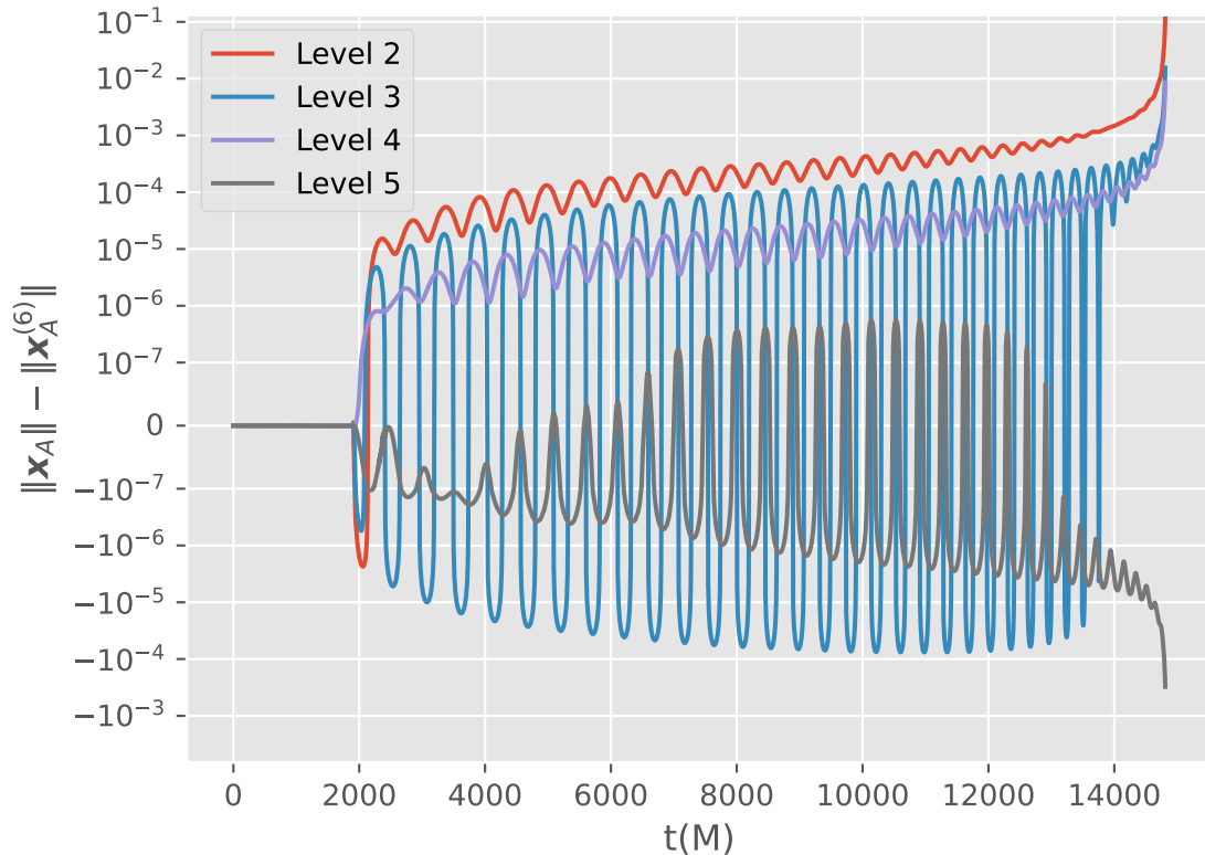
Difference in centers of black hole A for Sim11
