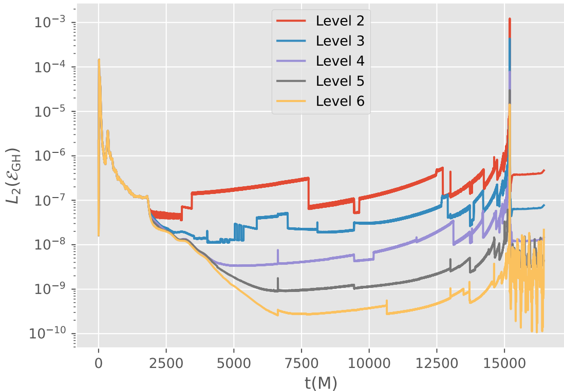
L_2(\mathcal{E}_{GH}) vs t(M) for Sim09
