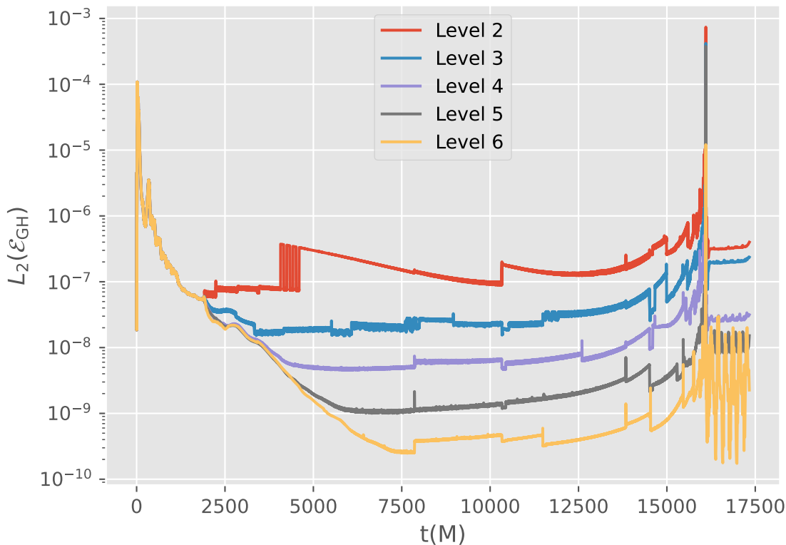
L_2(\mathcal{E}_{\text{GH}}) vs t(\text{M}) for Sim10
