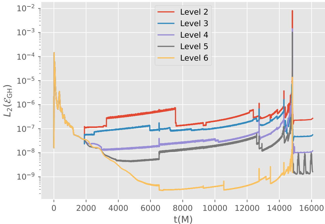
L_2(\mathcal{E}_{\text{GH}}) vs t(\text{M}) for Sim11
