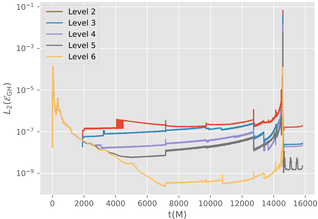
L_2(\mathcal{E}_{\text{GH}}) vs t(\text{M}) for Sim12
