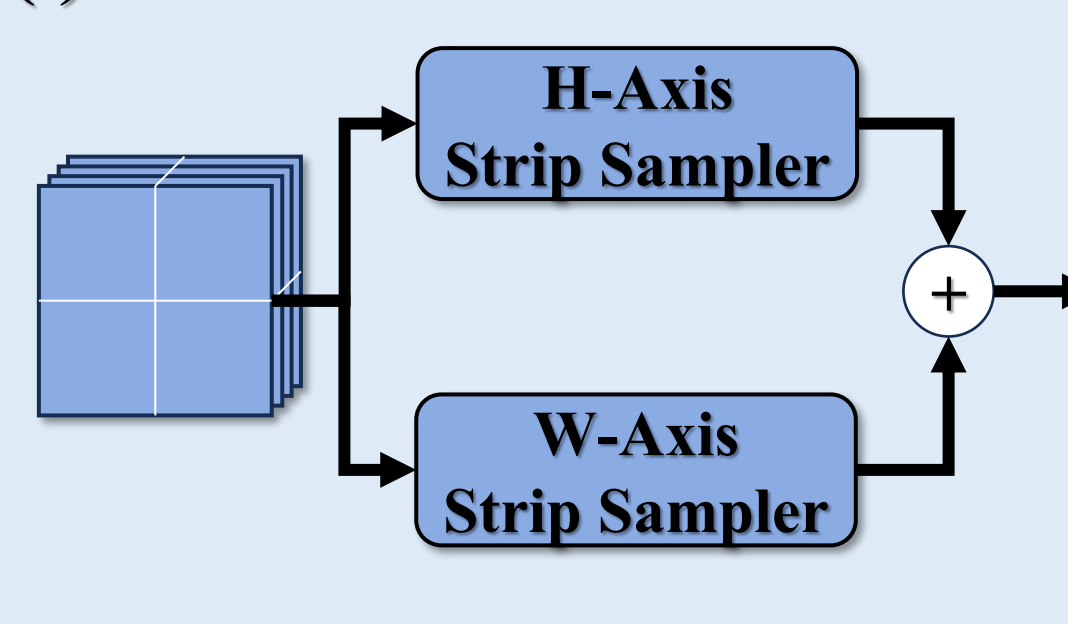
(f) 2D-CAConv
