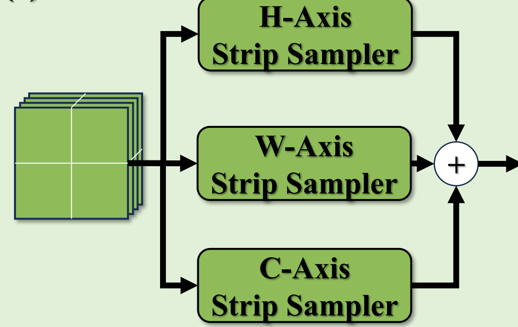
(e) 3D-CAConv
