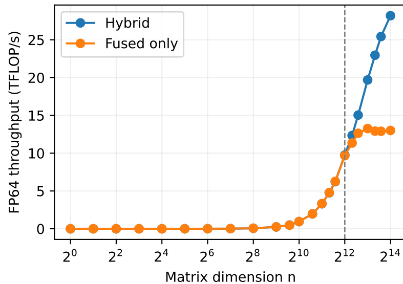
MI300A: FP64 no-pivot LU hybrid ablation Medians; shaded range = trial range
