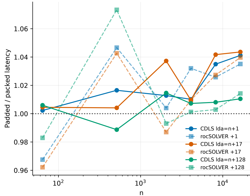
Leading-dimension sensitivity
