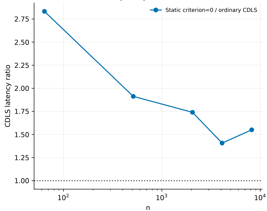
Static-pivot path overhead
