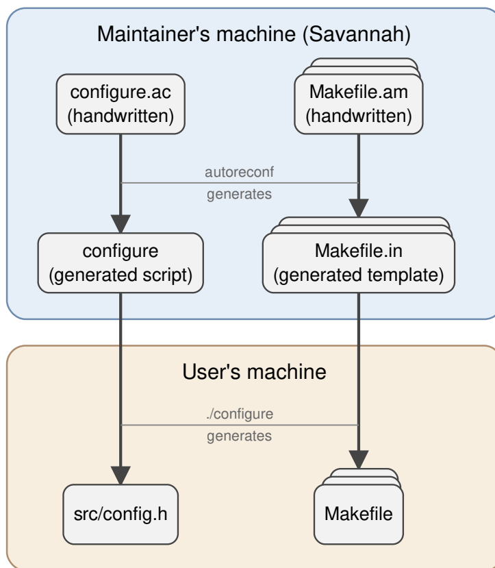
Figure 2. The Autotools build flow
