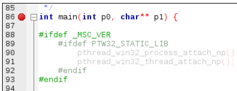
Abb. 6: Setzen von Breakpoints in Code::Blocks
