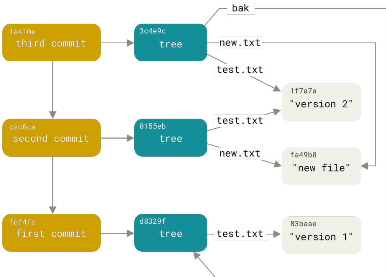
Figure 170. All the reachable objects in your Git directory
