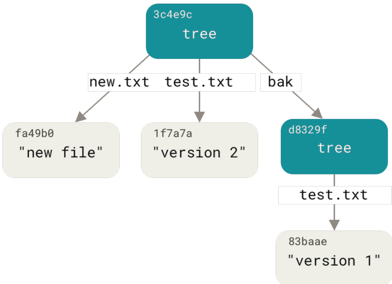
Figure 169. The content structure of your current Git data
