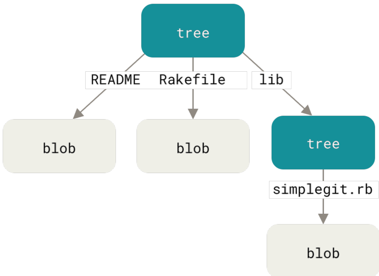
Figure 168. Simple version of the Git data model
