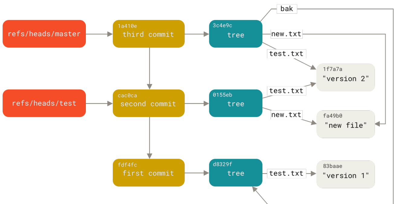
Figure 171. Git directory objects with branch head references included
