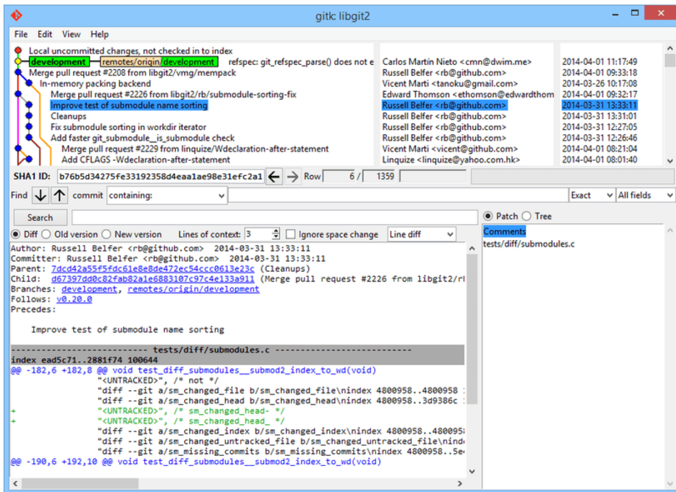
Figure 172. The gitk history viewer
