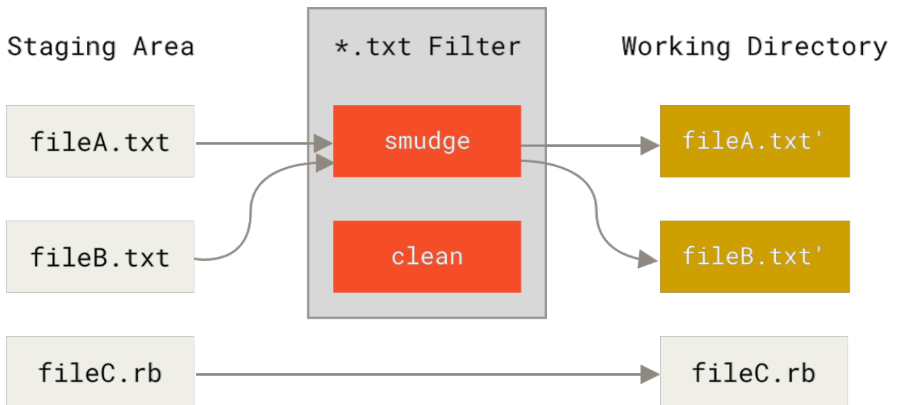
Figure 164. The “smudge” filter is run on checkout
