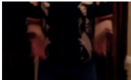
H-SSIM 0.423
