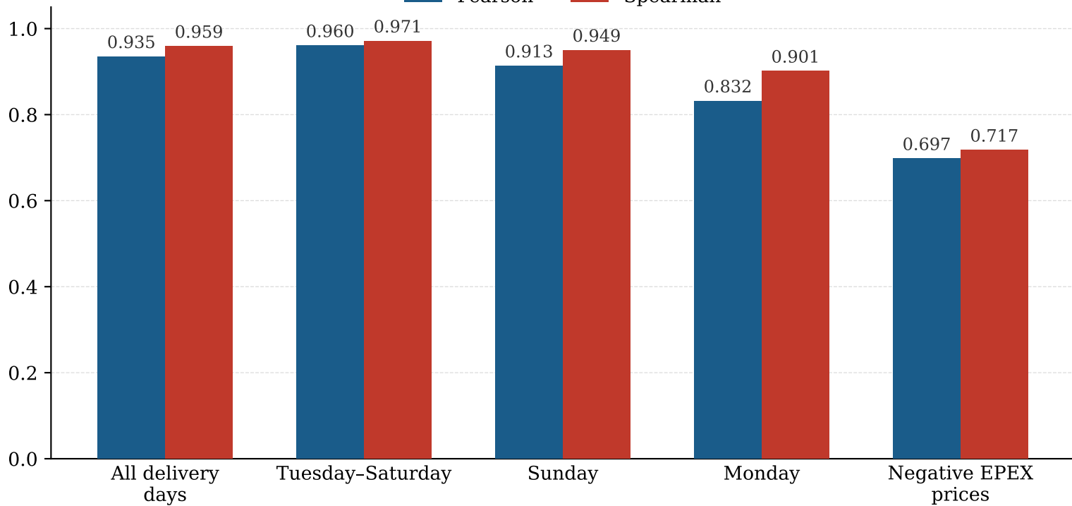
Correlation coefficient
