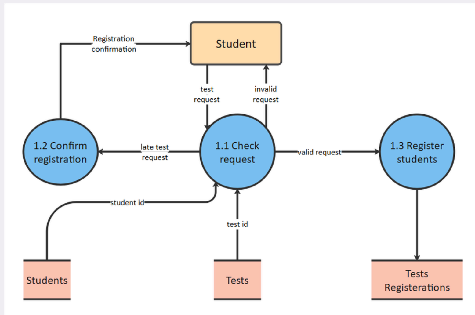
Figure1 - DFD Example
