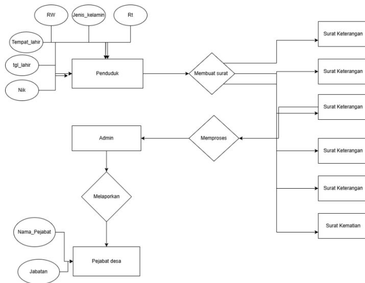
Gambar 3. 1 Diagram erd
