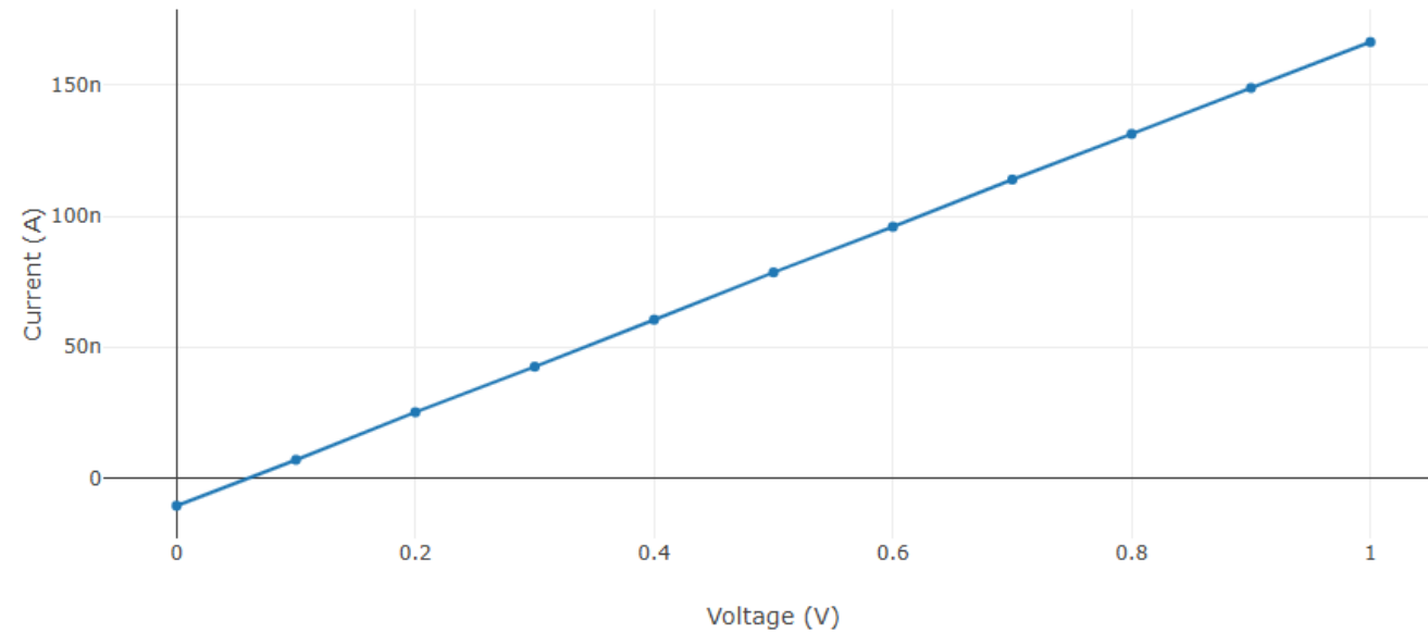
I-V Curve
