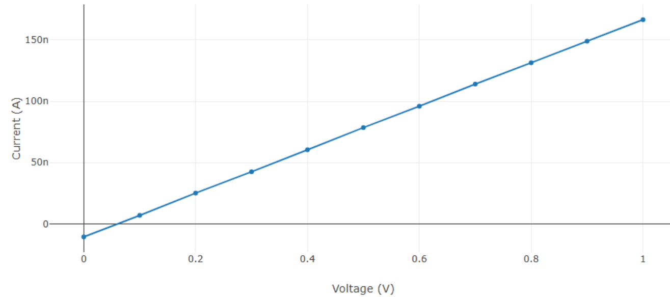
I-V Curve
