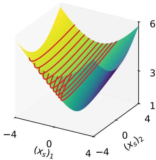
Lorentz
