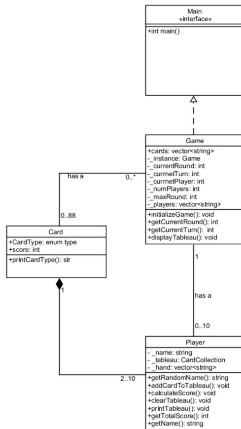
Class Diagram
