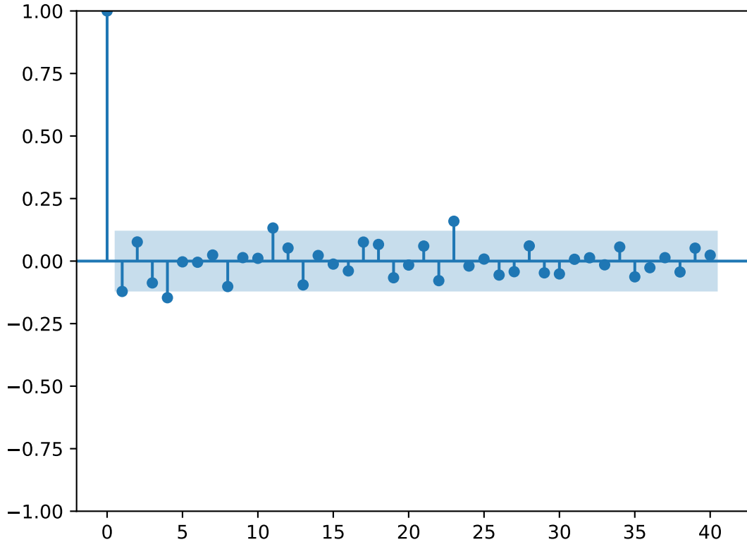
PACF - Differenced Series
