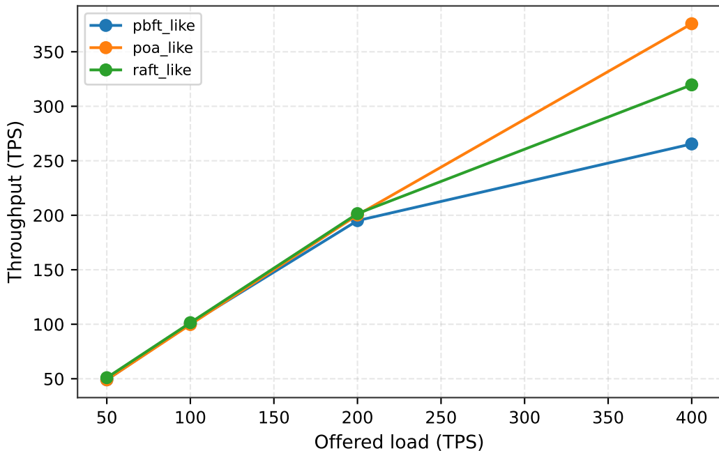
Consensus Throughput vs Load
