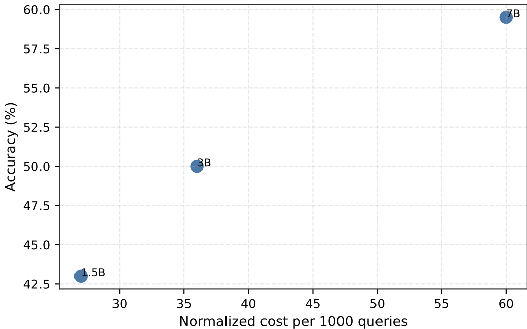
Backbone Cost-Accuracy Tradeoff
