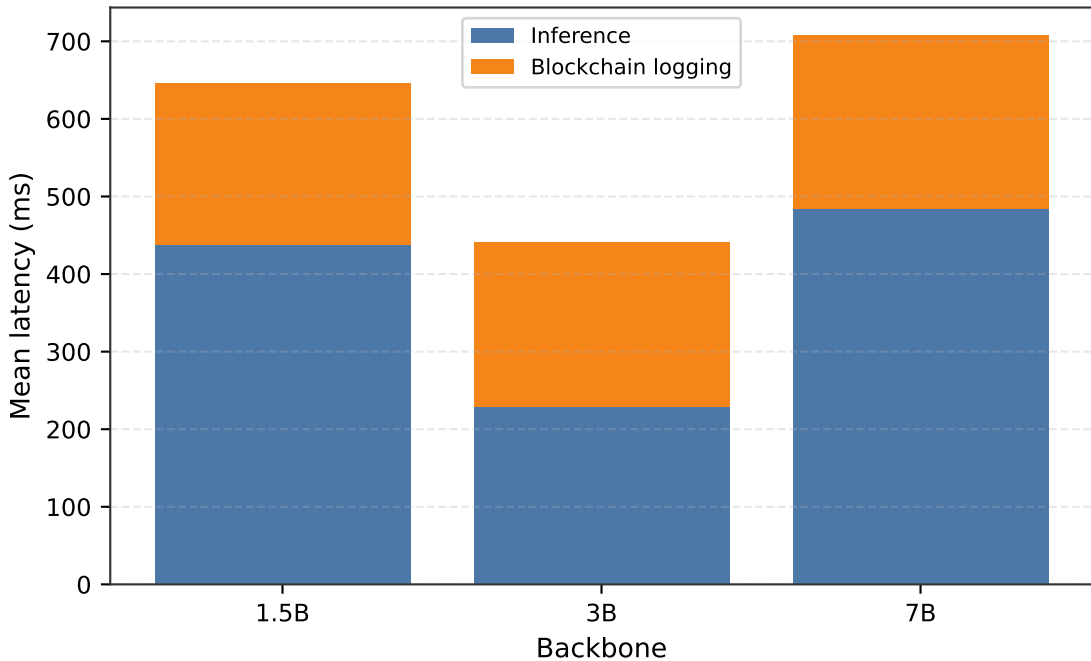
Real Backbone Latency Breakdown
