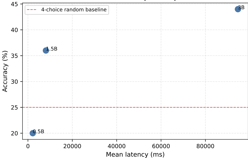
Real Backbone Accuracy-Latency Tradeoff
