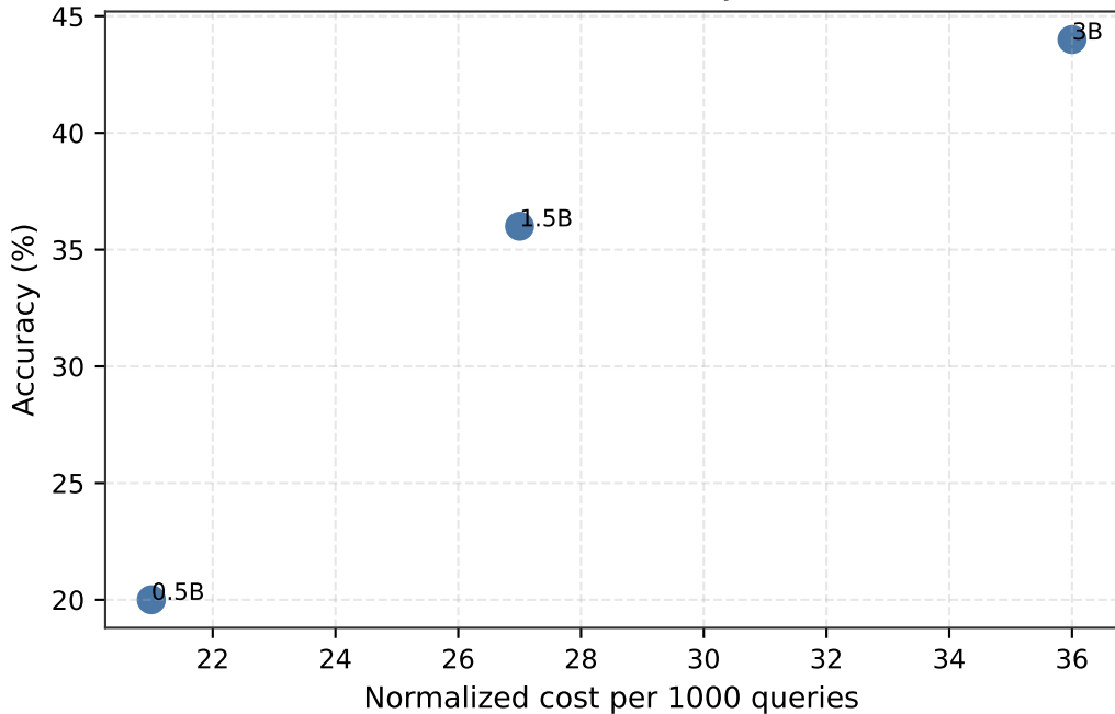
Backbone Cost-Accuracy Tradeoff
