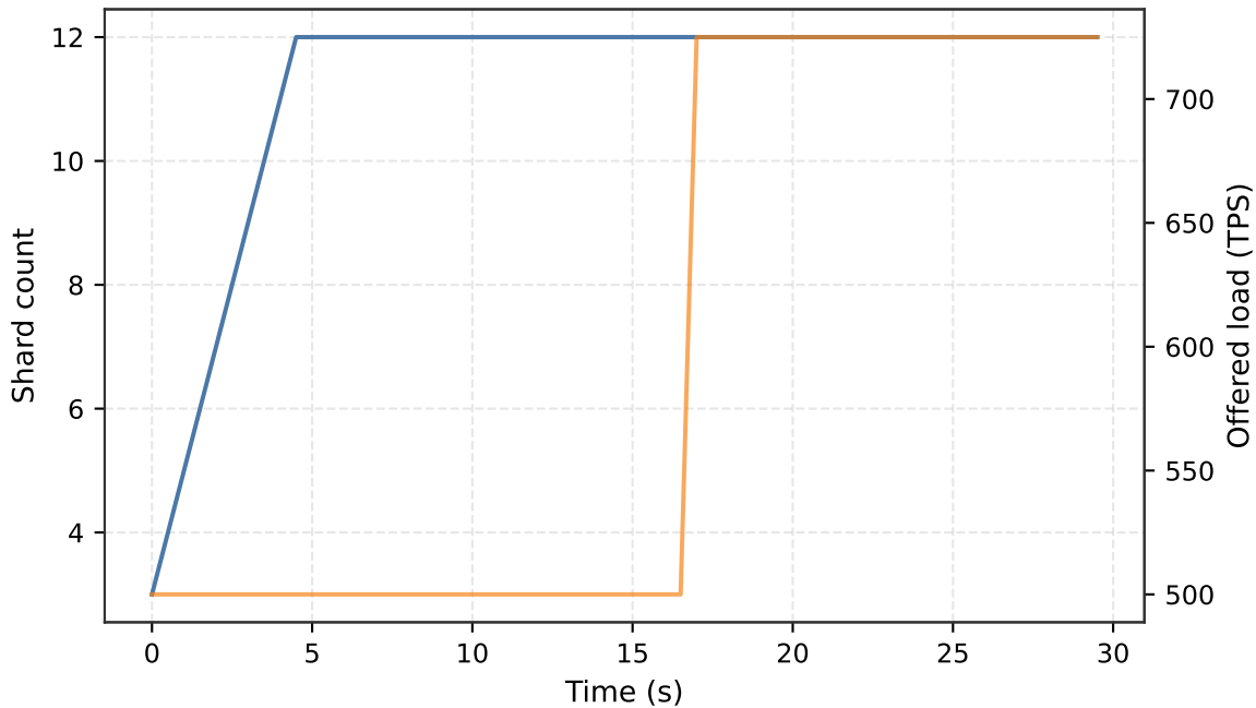
Dynamic Shard Adaptation
