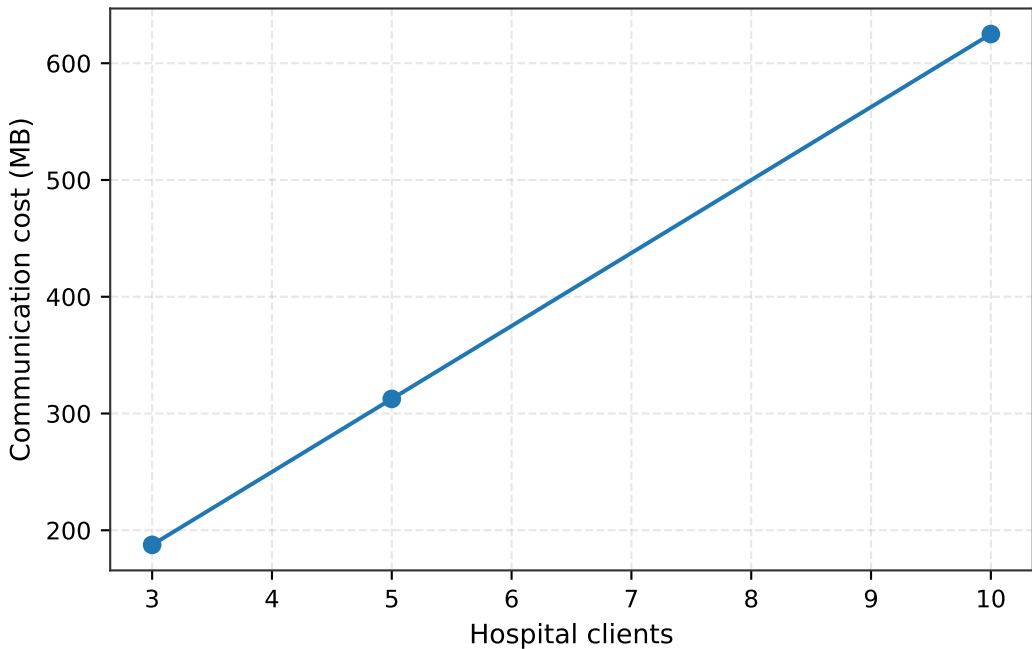
FL Client Scalability
