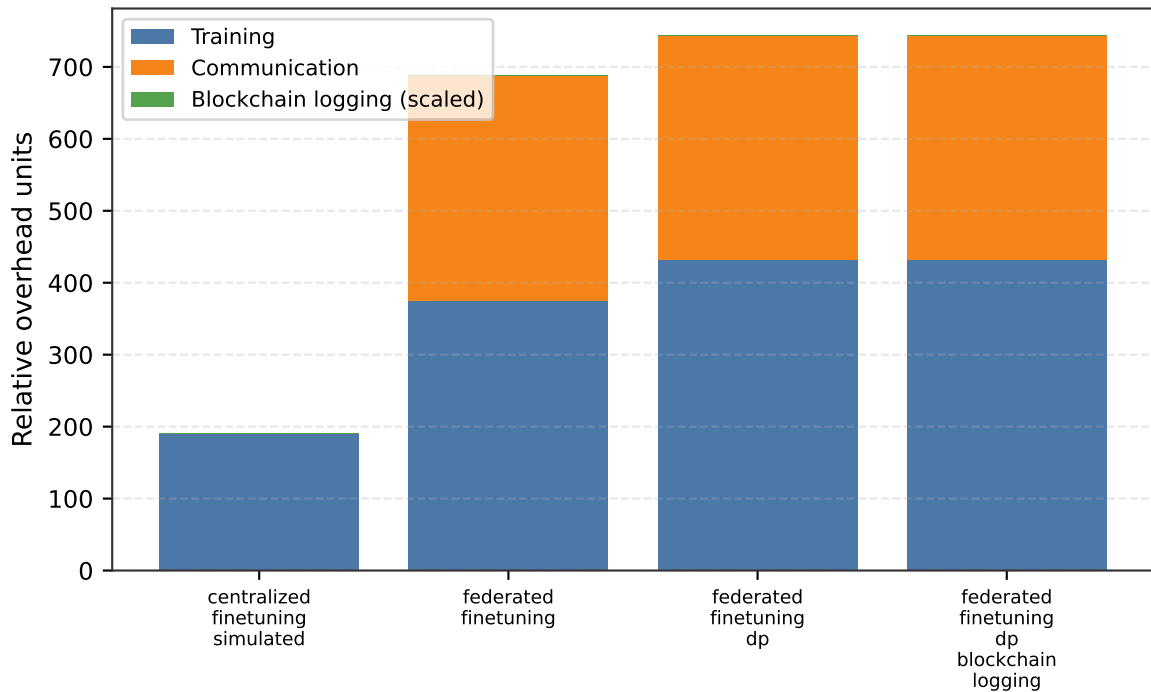
FL Overhead Breakdown
