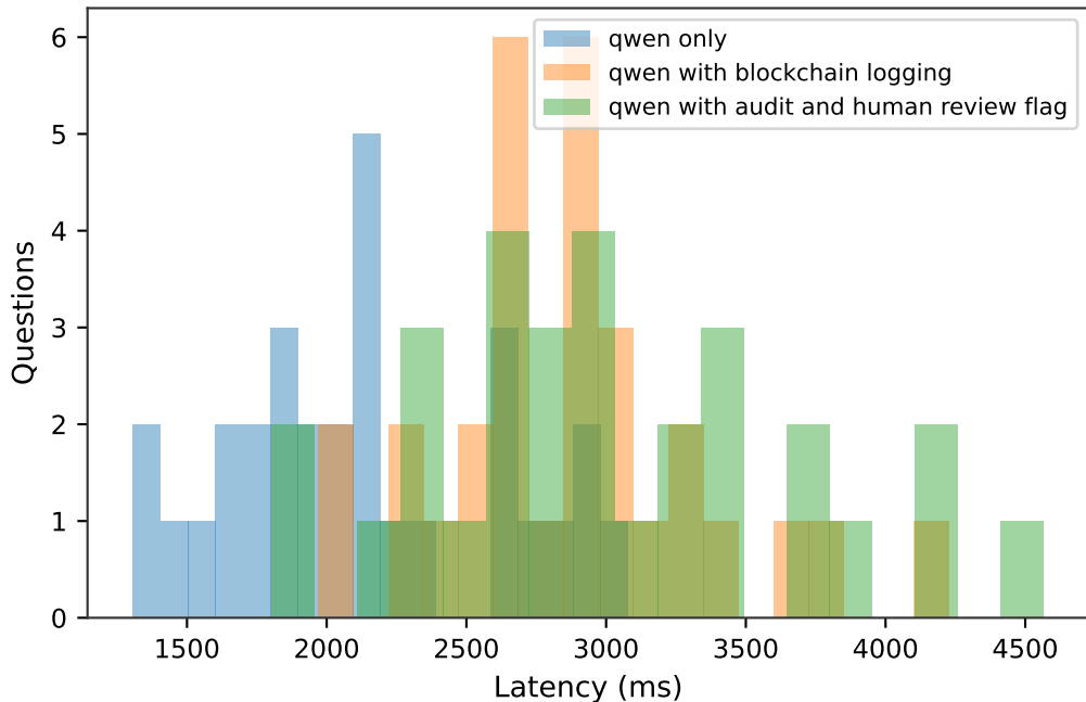
MedQA Latency Distribution
