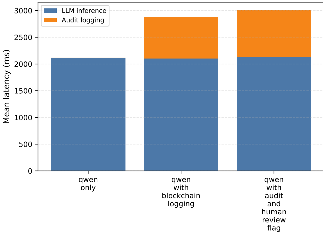
MedQA Workflow Overhead Breakdown
