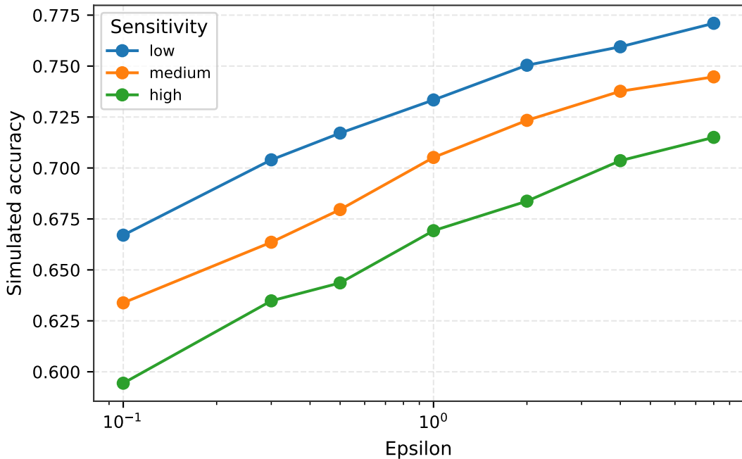
Privacy-Utility Tradeoff
