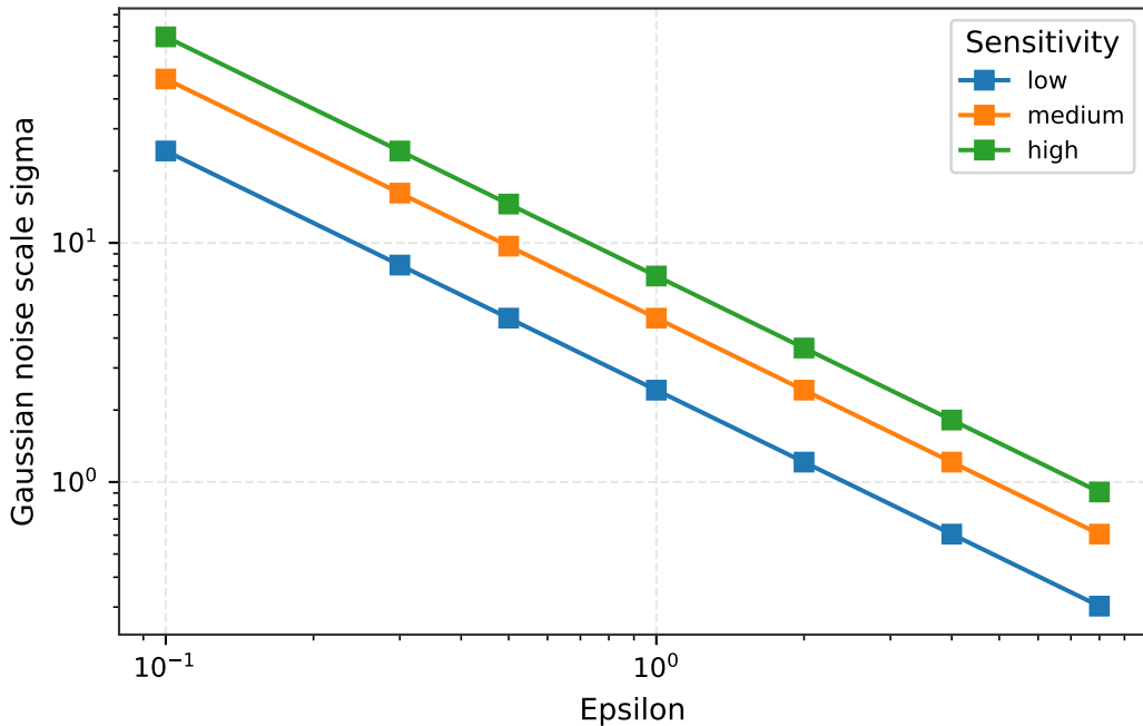
Noise Scale vs Epsilon
