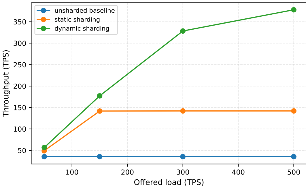
Throughput vs Offered Load
