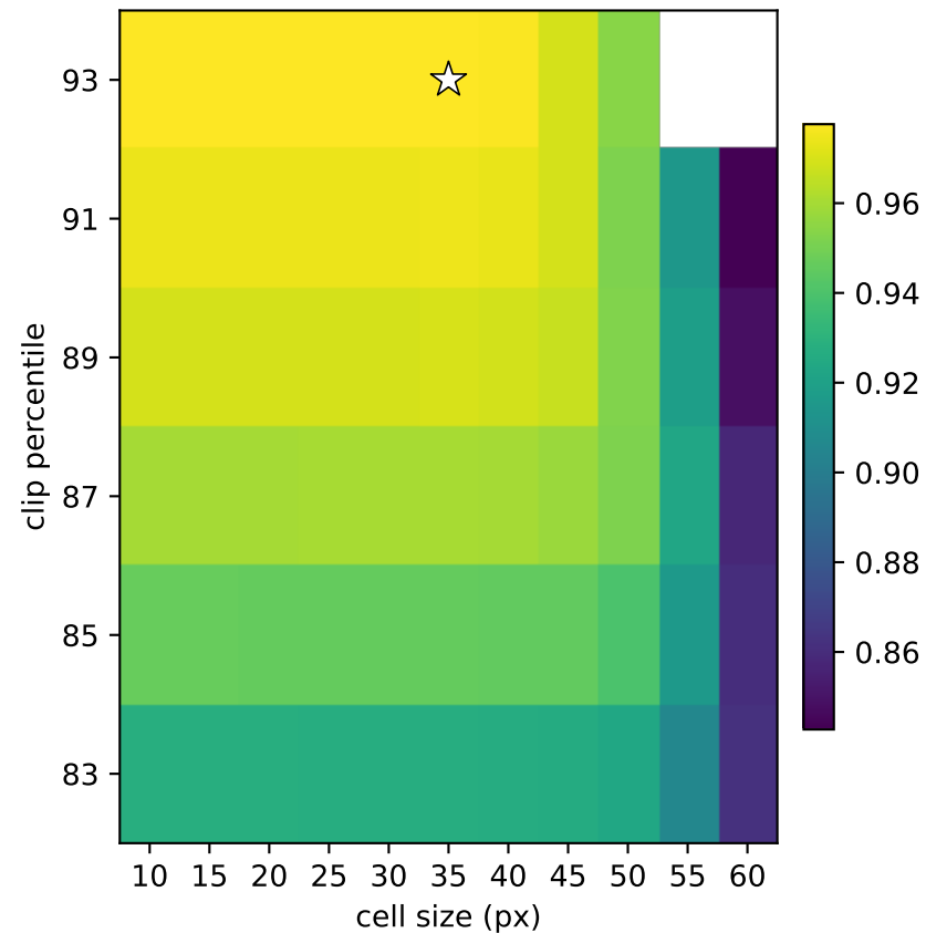
DET (max = 0.9776 @ 93, 35)
