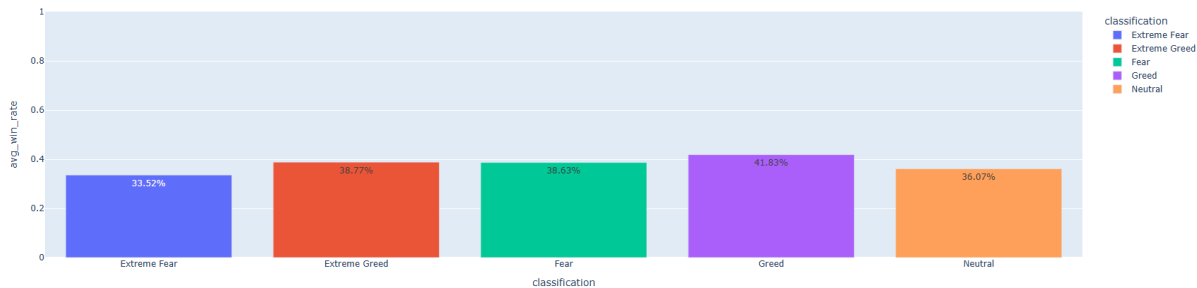
Average Win Rate by Market Sentiment
