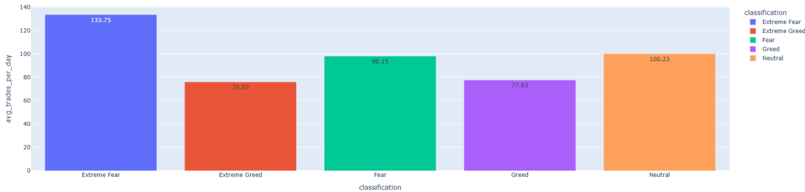
Average Number of Trades per Day by Market Sentiment
