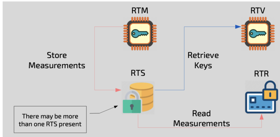
Figure 1.1: TPM Architecture and Roots of Trust
