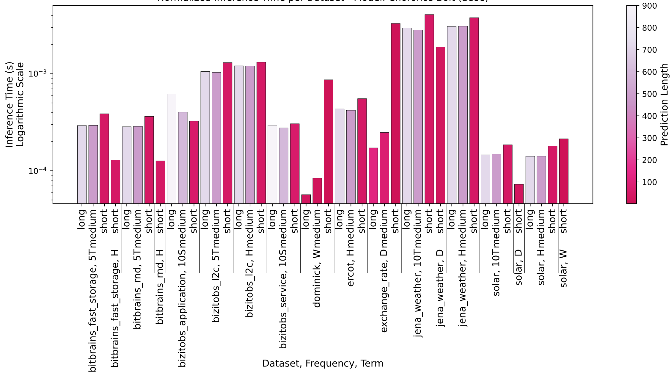
Normalized Inference Time per Dataset - Model: Choronos Bolt (Base)
