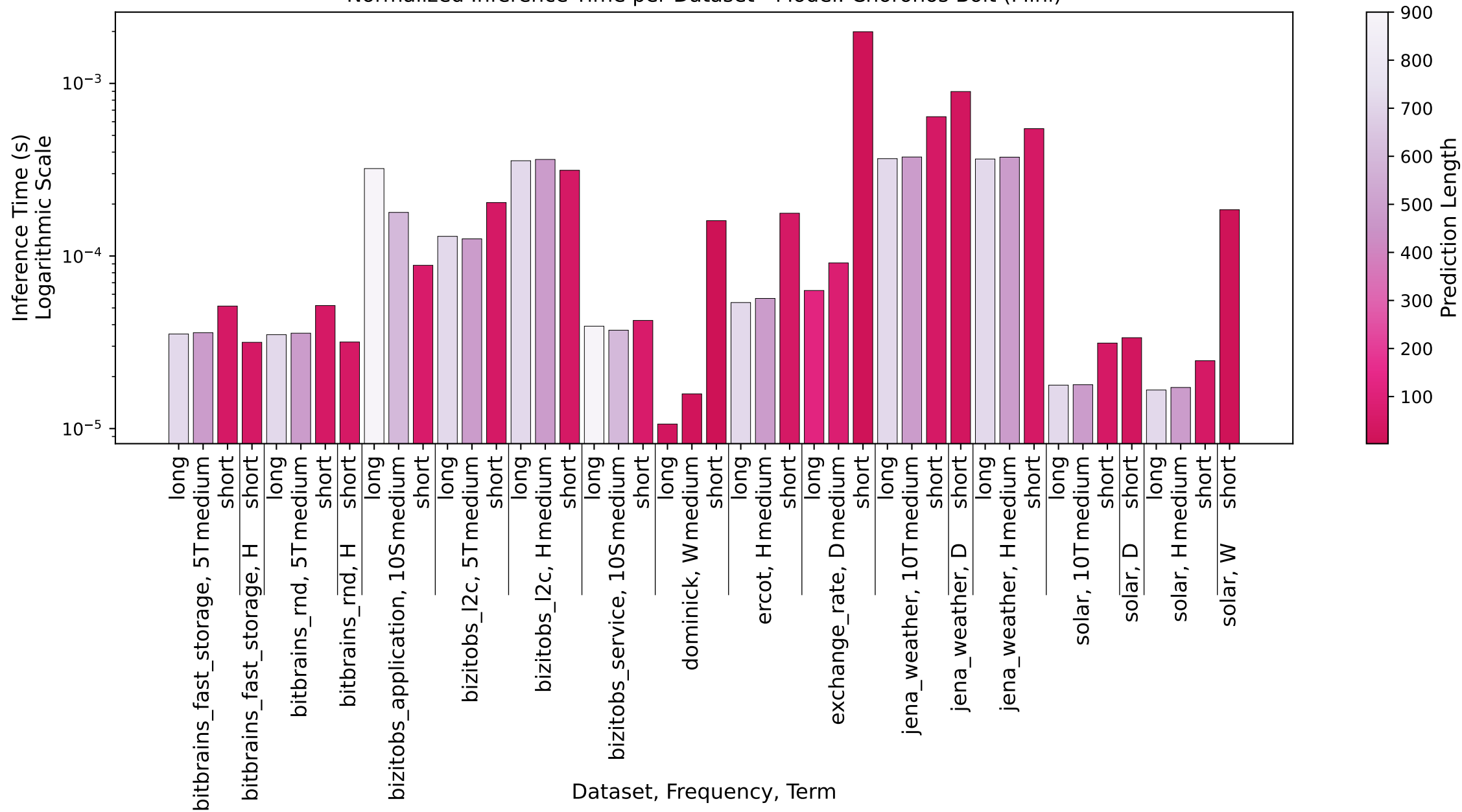
Normalized Inference Time per Dataset - Model: Chronos Bolt (Mini)
