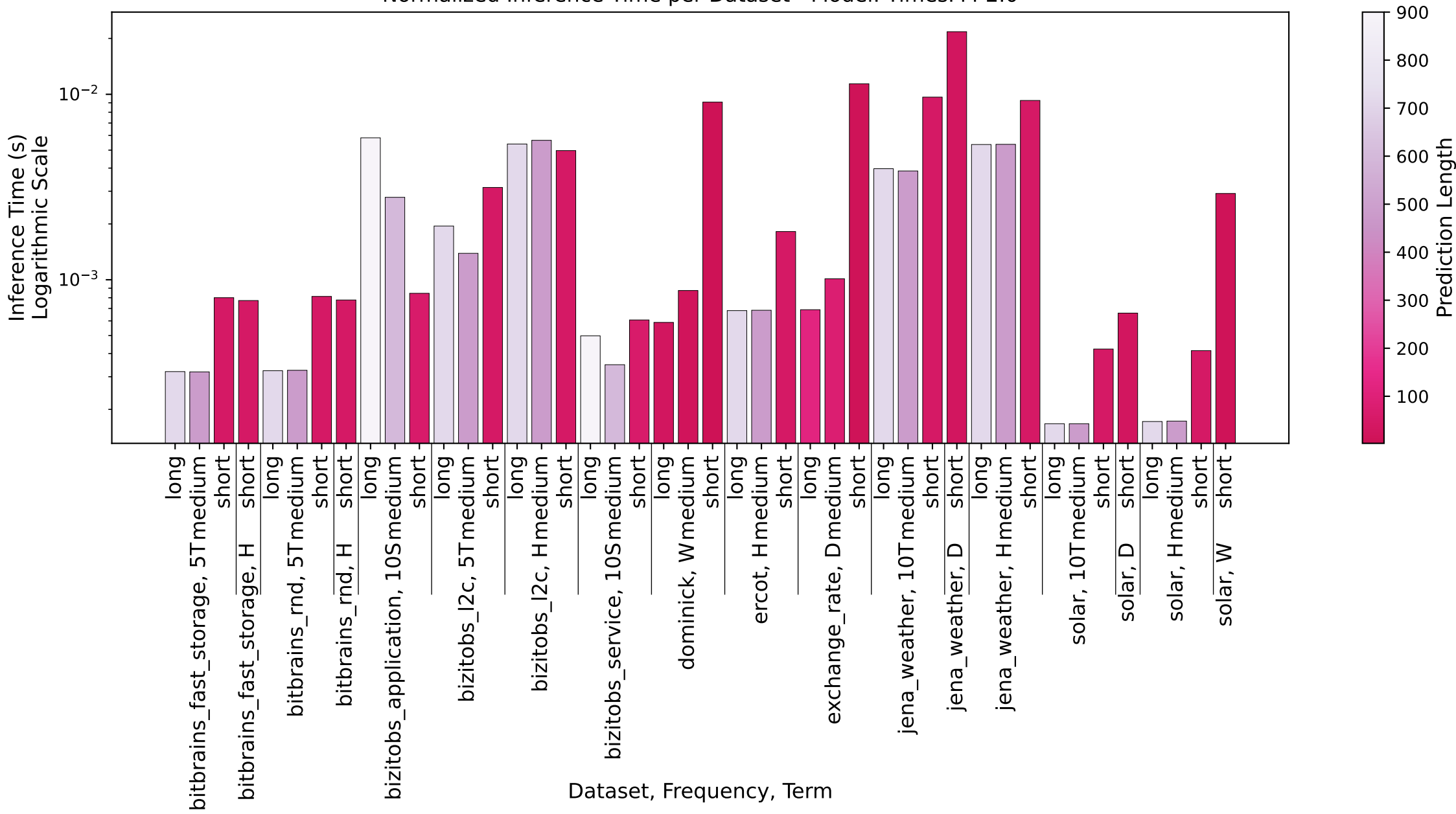
Normalized Inference Time per Dataset - Model: TimesFM-2.0
