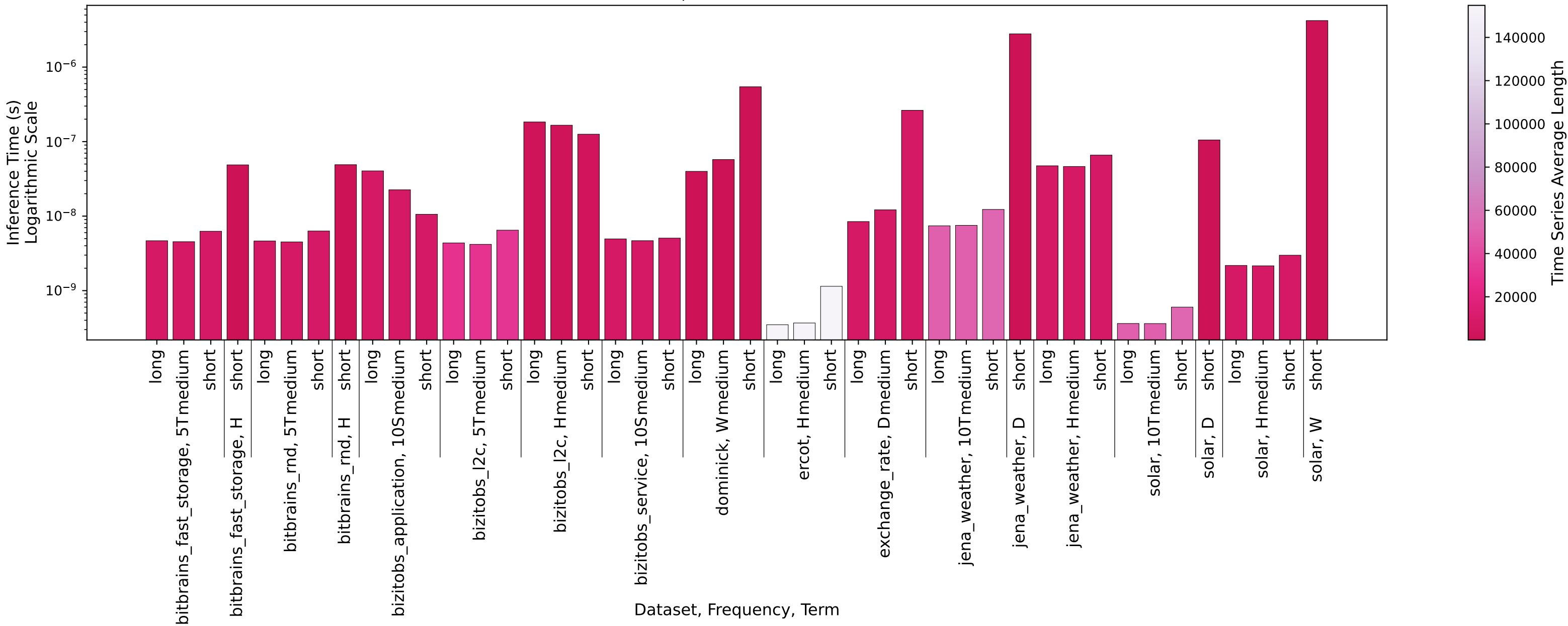
Normalized Inference Time per Dataset - Model: Choronos Bolt (Mini)
