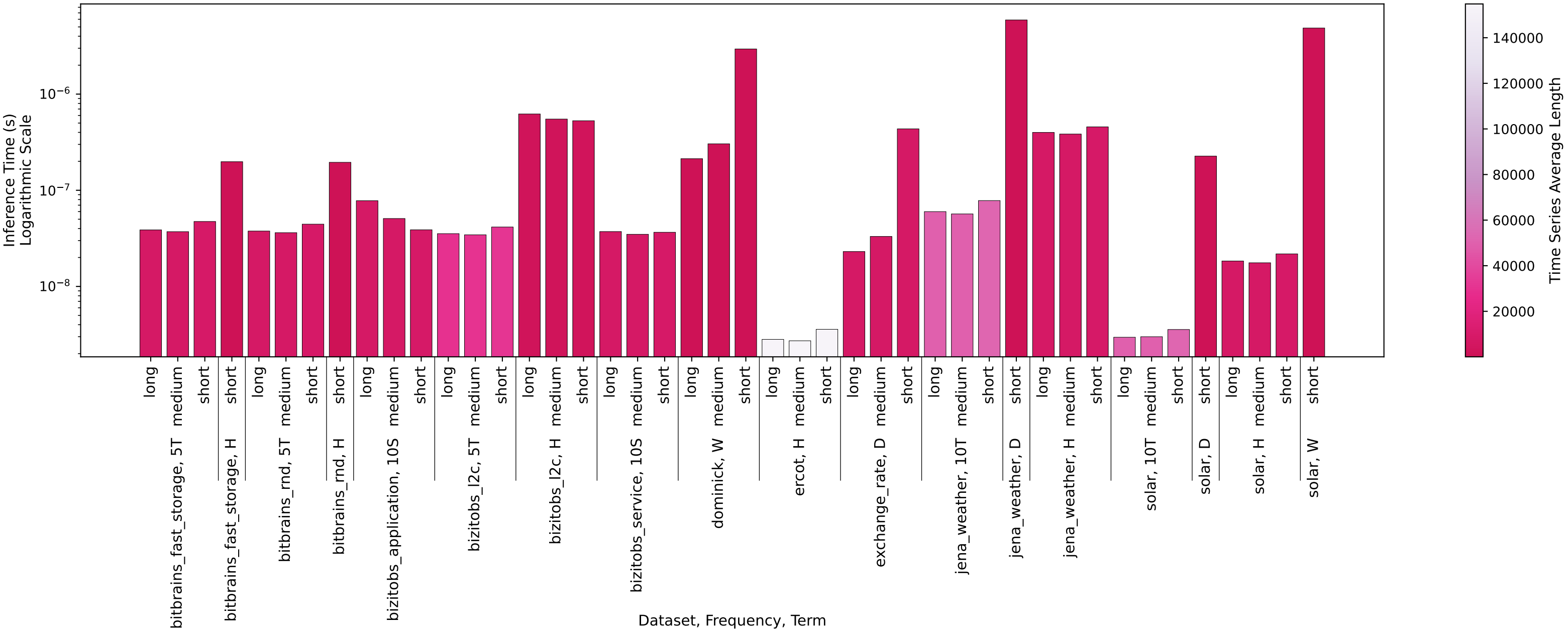
Normalized Inference Time per Dataset - Model: Choronos Bolt (Base)
