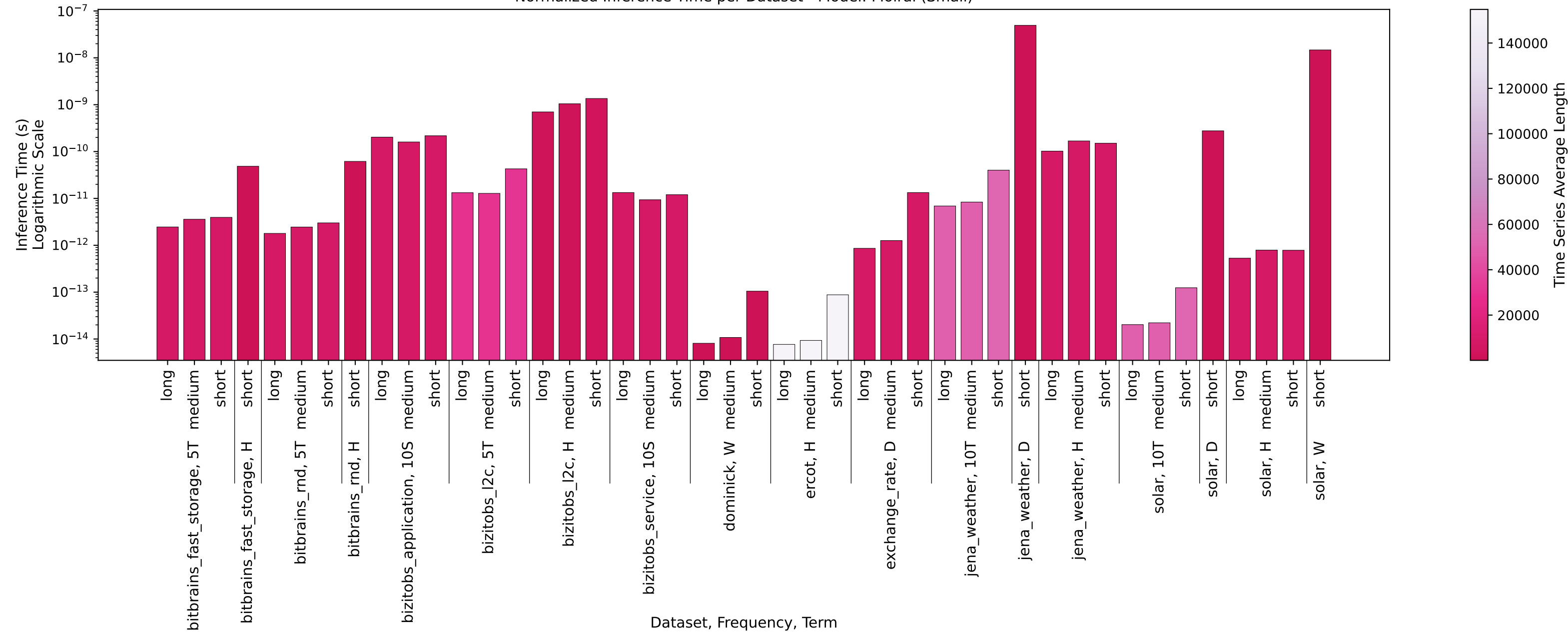
Normalized Inference Time per Dataset - Model: Moirai (Small)
