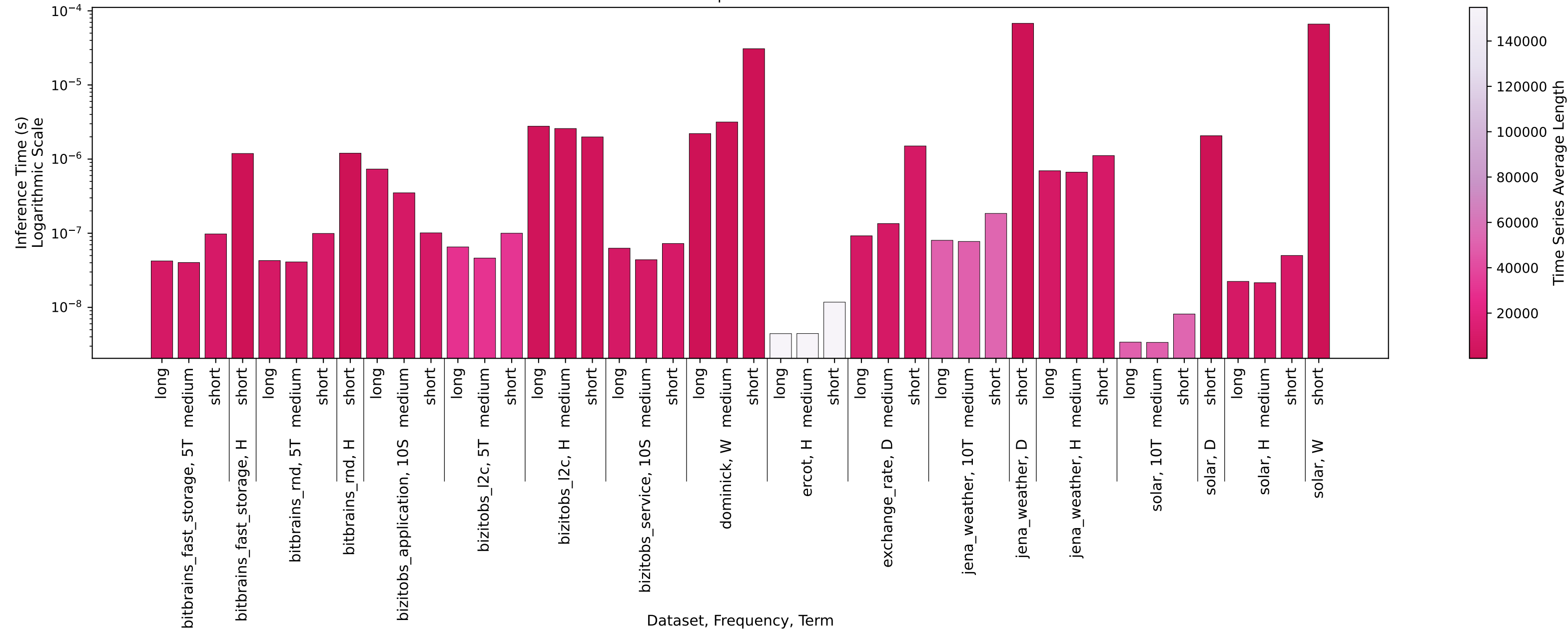
Normalized Inference Time per Dataset - Model: TimesFM-2.0
