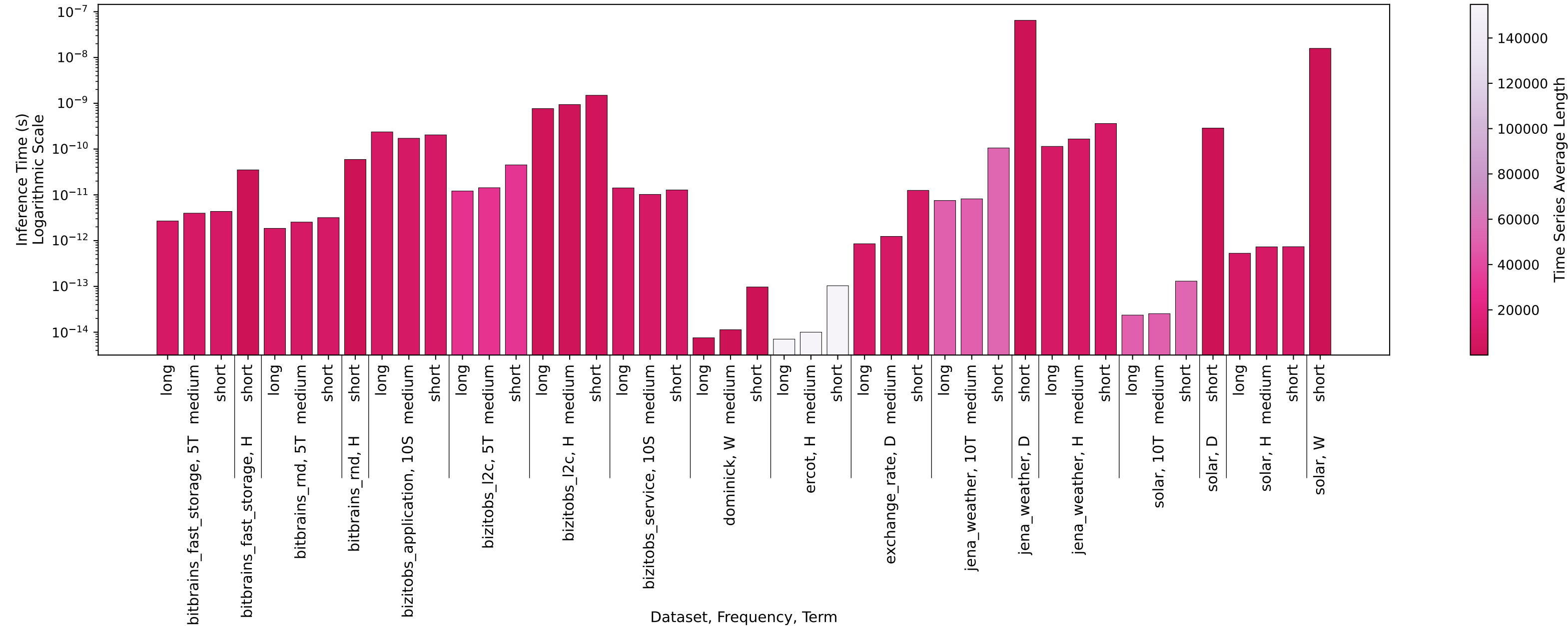
Normalized Inference Time per Dataset - Model: Moirai (Large)
