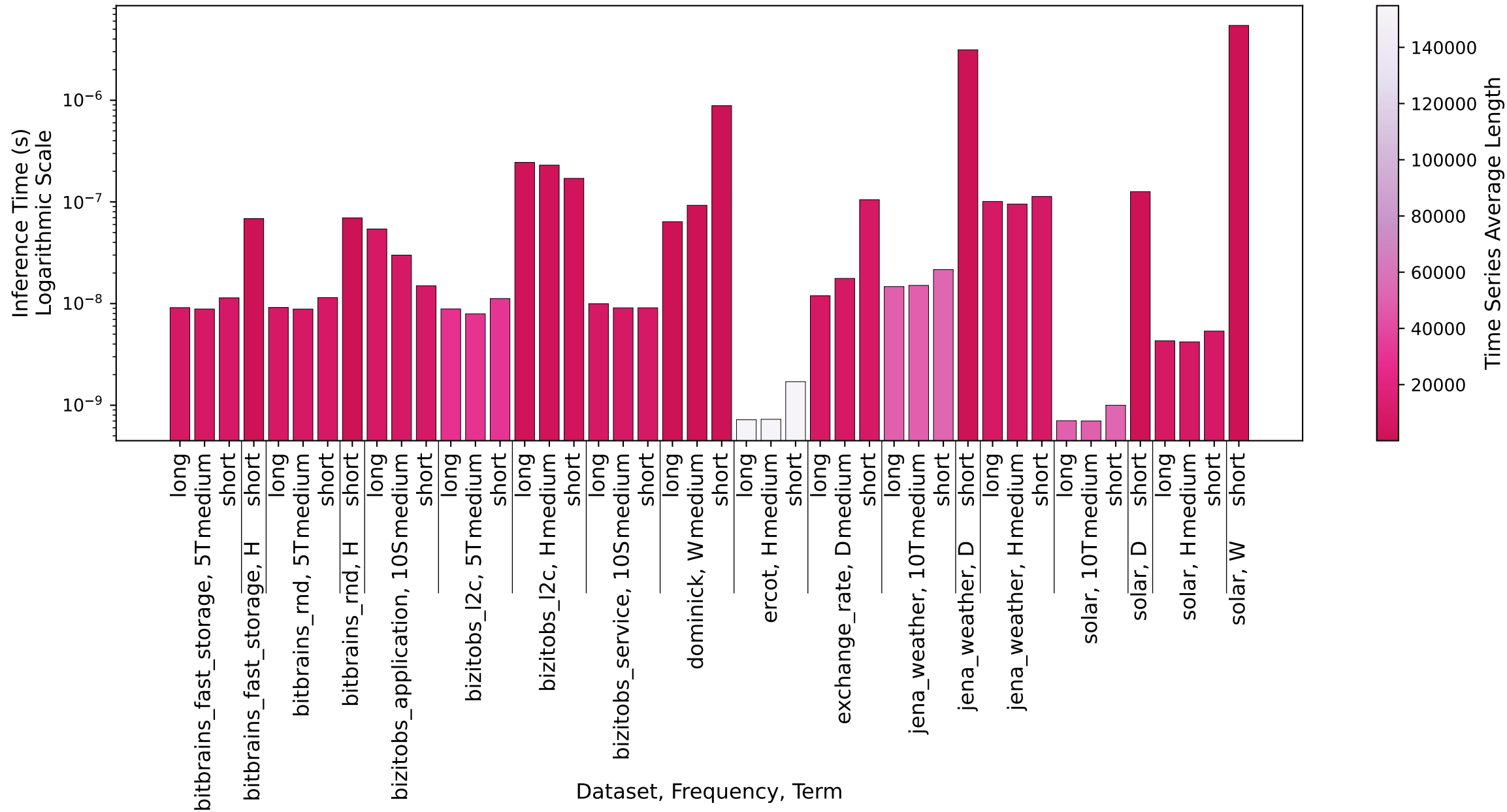
Normalized Inference Time per Dataset - Model: Choronos Bolt (Small)
