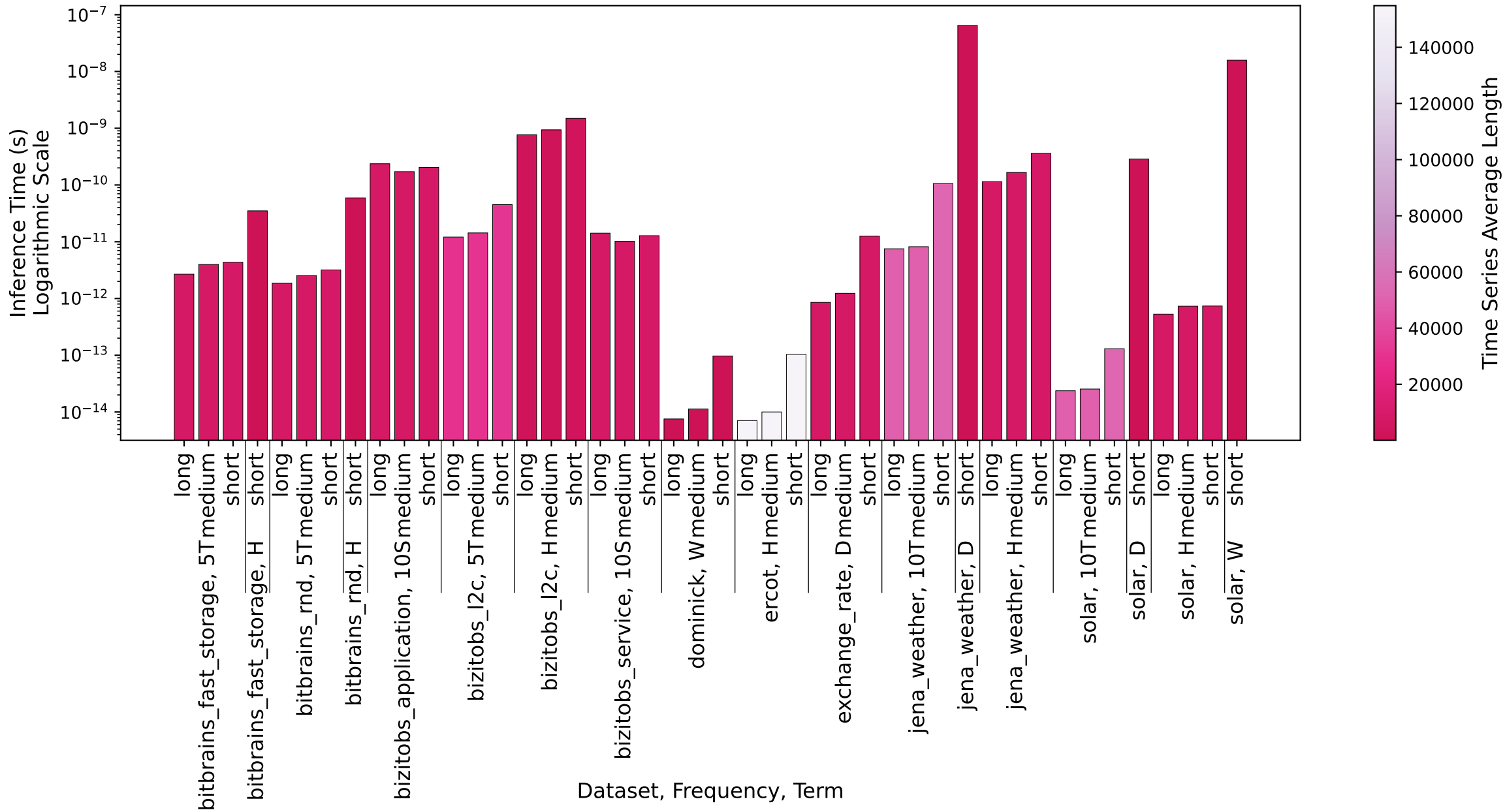
Normalized Inference Time per Dataset - Model: Moirai (Large)
