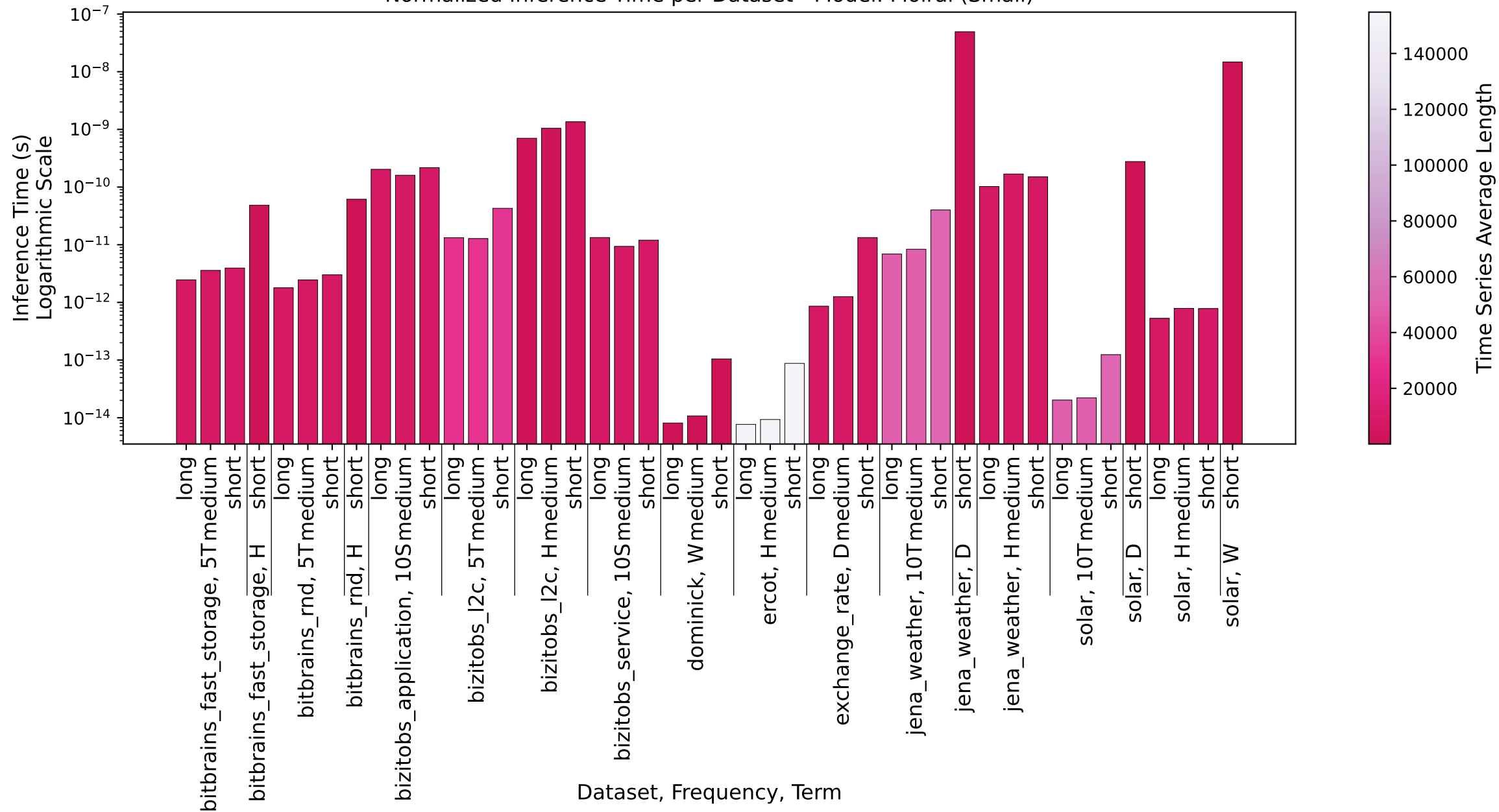
Normalized Inference Time per Dataset - Model: Moirai (Small)
